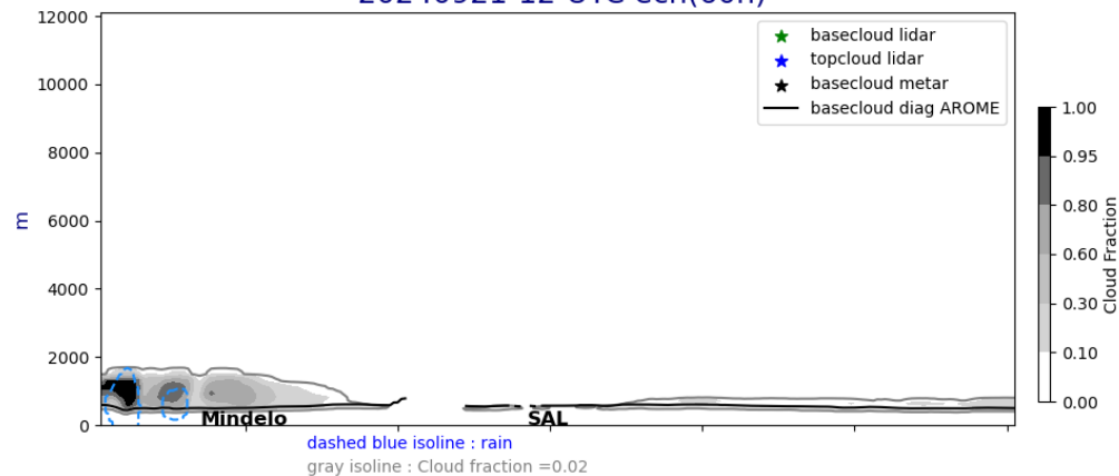
Cross section E/W @ 17.5N 20240921-12-UTC ech(60h)
