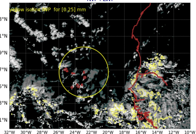
AROME25 20240921-12-UTC -ech(60h) IWP+LWP
