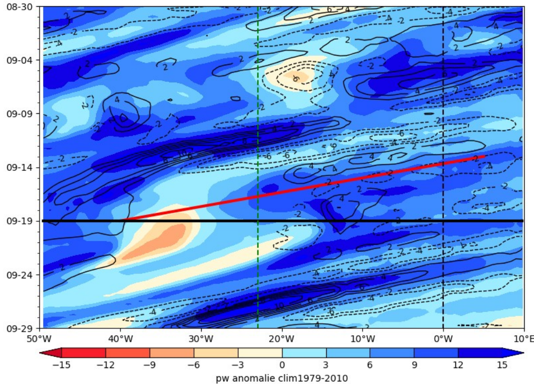
ECMWF PW (color) AND V at 925 hPa 2024-09-19
