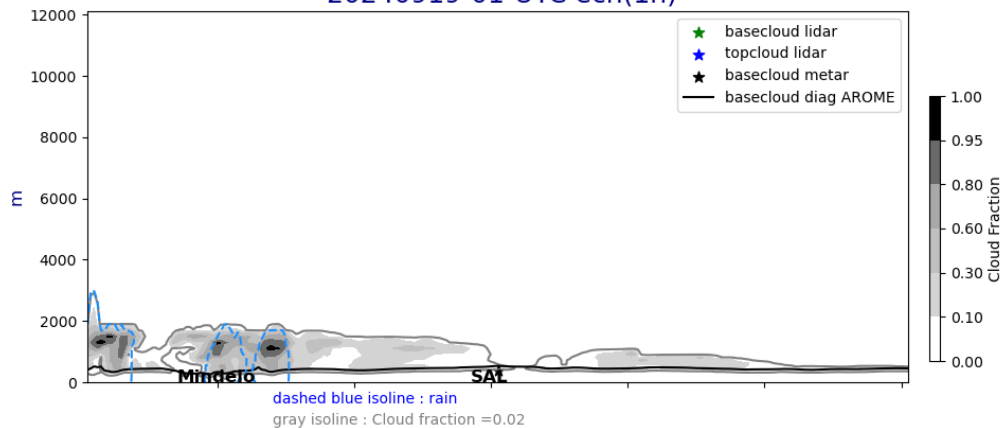
Cross section E/W @ 17.5N 20240919-01-UTC ech(1h)
