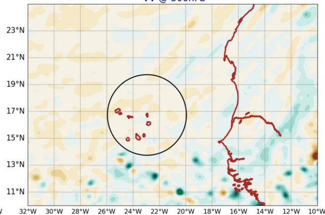
AROME25 20240920-12-UTC -ech(36h) VV @ 500hPa
