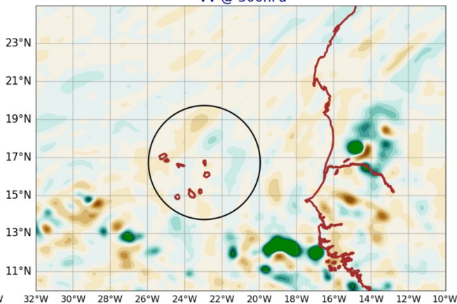
AROME25 20240921-12-UTC -ech(60h) VV @ 500hPa
