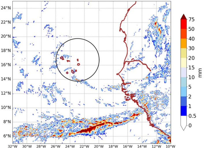
AROME25 20240919-15-UTC -ech(15h) RR cumulated over 6h
