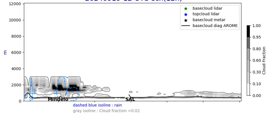
Cross section E/W @ 17.5N 20240919-12-UTC ech(12h)
