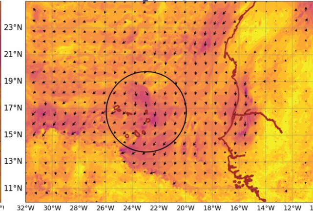
AROME25 20240920-12-UTC -ech(36h) wind_sp920 @ 920hPa
