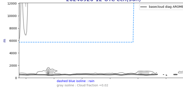
Cross section S/N @ -22W 20240920-12-UTC ech(36h)
