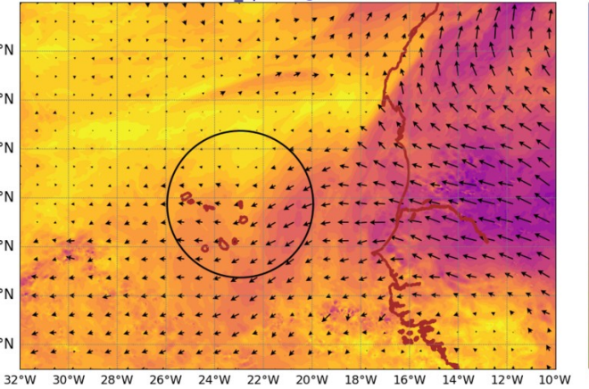
AROME25 20240921-12-UTC -ech(60h) wind_sp920 @ 920hPa
