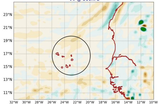
AROME25 20240919-12-UTC -ech(12h) VV @ 500hPa
