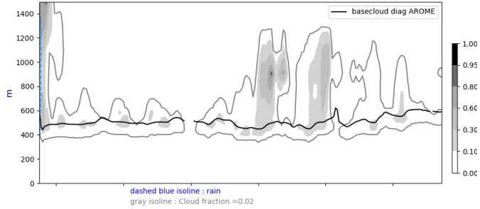
Cross section S/N @ -22W 20240919-12-UTC ech(12h)
