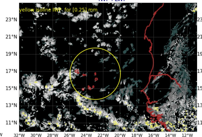
AROME25 20240920-12-UTC -ech(36h) IWP+LWP
