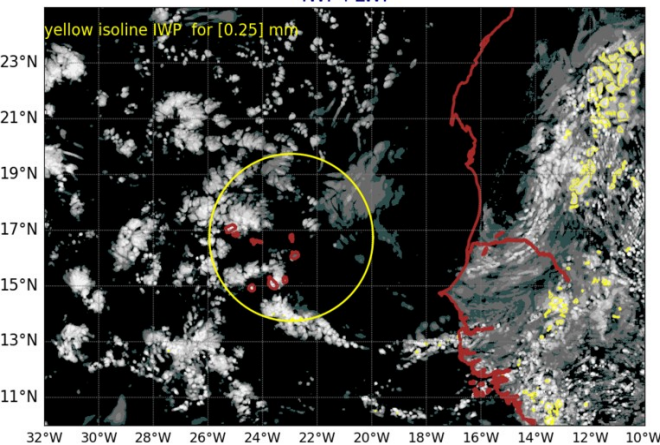
AROME25 20240919-12-UTC -ech(12h) IWP+LWP
