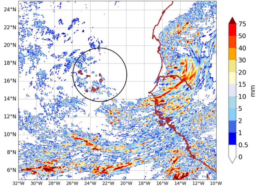
AROME25 20240919-00-UTC -ech(24h)
