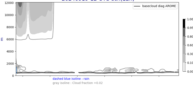
Cross section S/N @ -22W 20240919-12-UTC ech(12h)
