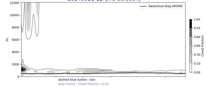
Cross section S/N @ -22W 20240921-12-UTC ech(60h)
