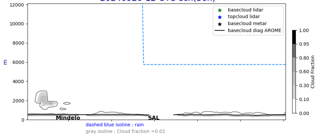
Cross section E/W @ 17.5N 20240920-12-UTC ech(36h)
