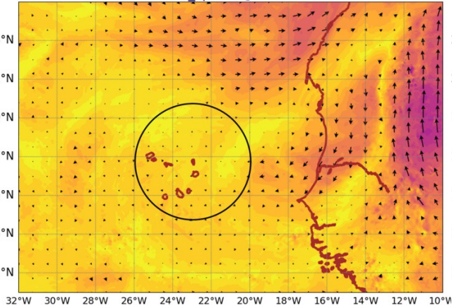
AROME25 20240919-12-UTC -ech(12h) wind_sp920 @ 920hPa
