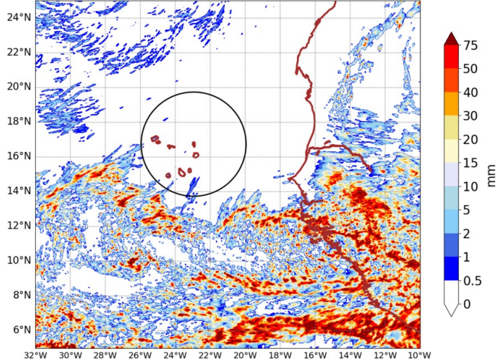
AROME25 20240921-12-UTC -ech(60h) RR cumulated over 24h
