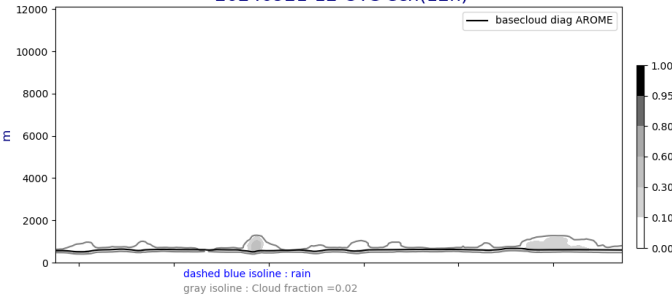
Cross section S/N @ -22W 20240921-12-UTC ech(12h)
