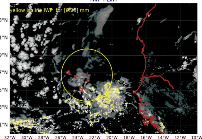
AROME25 20240923-12-UTC -ech(60h) IWP+LWP
