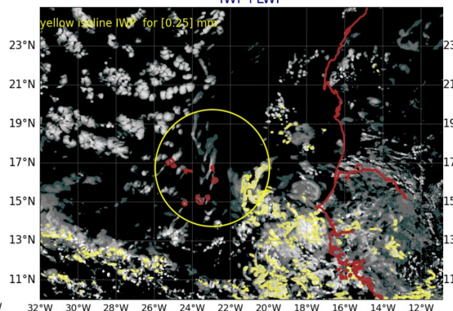
AROME25 20240922-12-UTC -ech(36h) IWP+LWP
