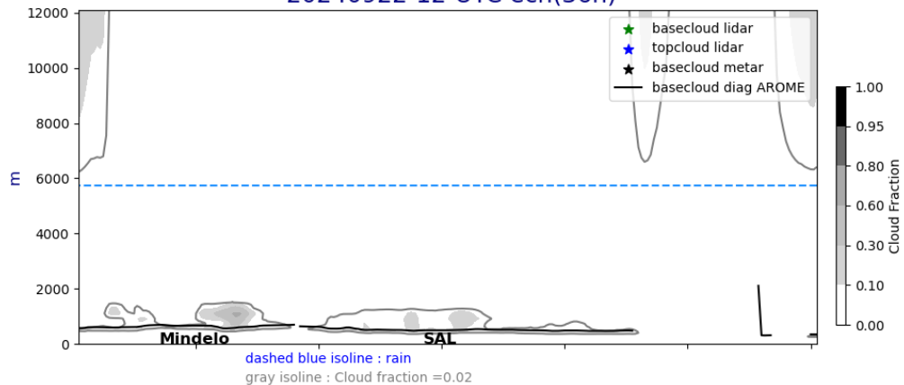
Cross section E/W @ 17.5N 20240922-12-UTC ech(36h)
