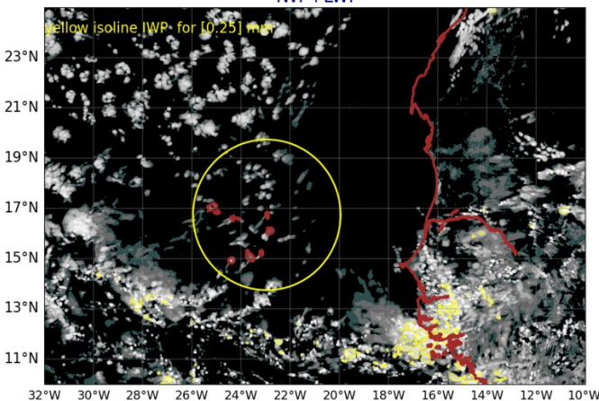
AROME25 20240921-12-UTC -ech(12h) IWP+LWP
