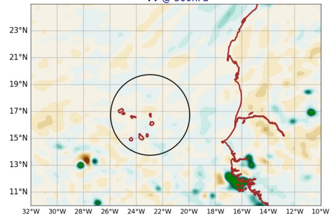
AROME25 20240921-12-UTC -ech(12h) VV @ 500hPa
