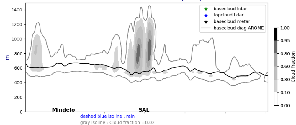
Cross section E/W @ 17.5N 20240921-12-UTC ech(12h)
