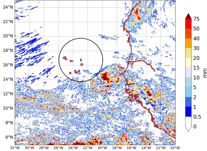
AROME25 20240923-12-UTC -ech(60h) RR cumulated over 24h
