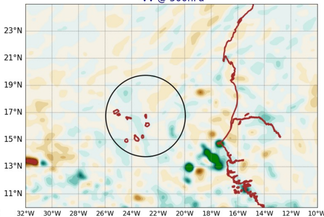
AROME25 20240922-12-UTC -ech(36h) VV @ 500hPa
