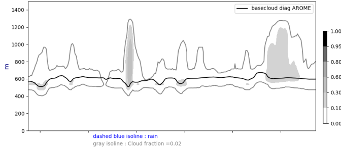
Cross section S/N @ -22W 20240921-12-UTC ech(12h)
