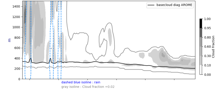
Cross section S/N @ -22W 20240923-12-UTC ech(60h)
