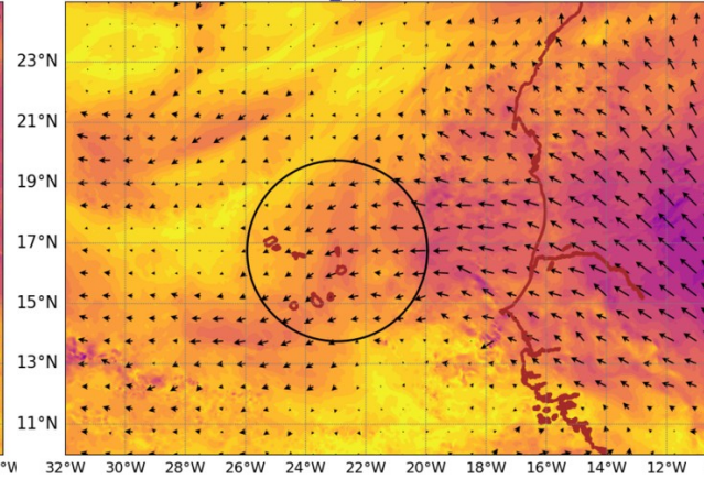
AROME25 20240922-12-UTC -ech(36h) wind_sp920 @ 920hPa
