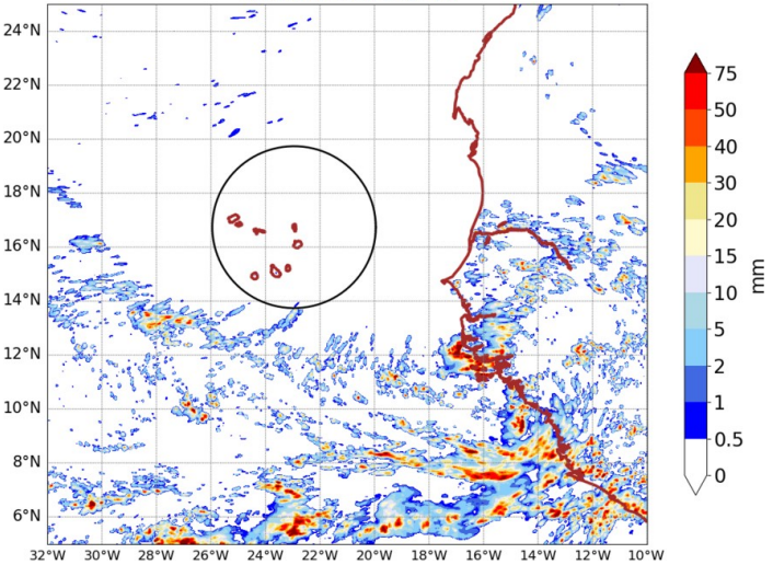
AROME25 20240921-15-UTC -ech(15h) RR cumulated over 6h
