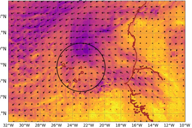
AROME25 20240923-12-UTC -ech(60h) wind_sp920 @ 920hPa
