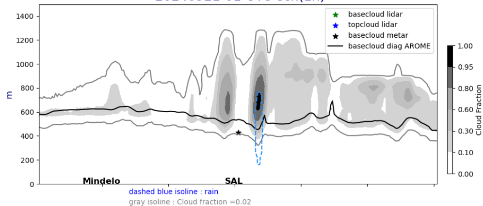
Cross section E/W @ 17.5N 20240921-01-UTC ech(1h)
