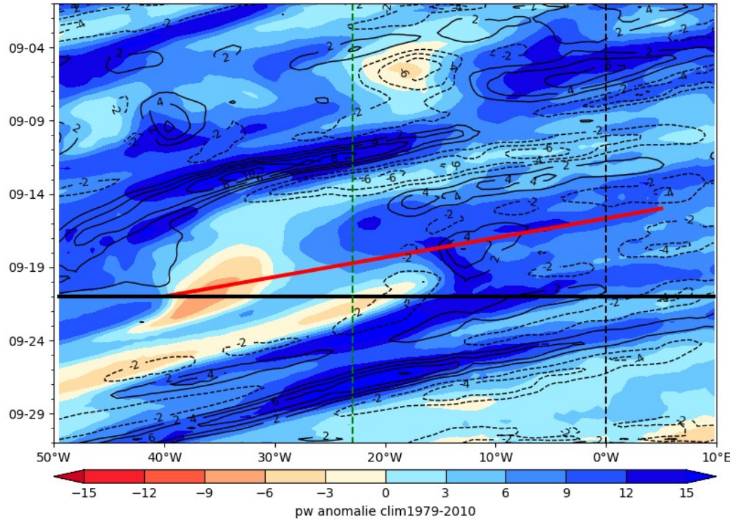
ECMWF PW (color) AND V at 925 hPa 2024-09-21
