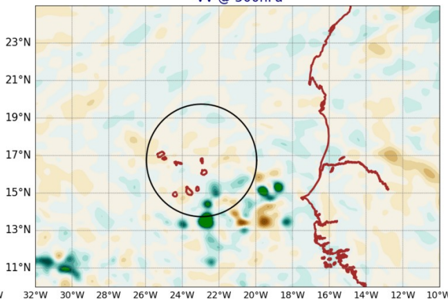
AROME25 20240923-12-UTC -ech(60h) VV @ 500hPa
