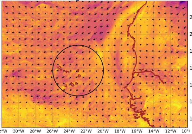
AROME25 20240921-12-UTC -ech(12h) wind_sp920 @ 920hPa
