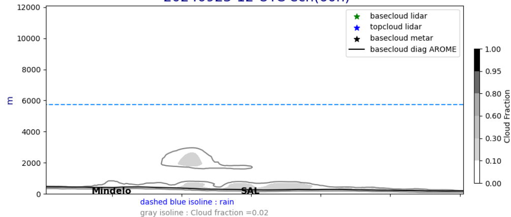
Cross section E/W @ 17.5N 20240923-12-UTC ech(60h)
