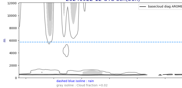
Cross section S/N @ -22W 20240922-12-UTC ech(36h)
