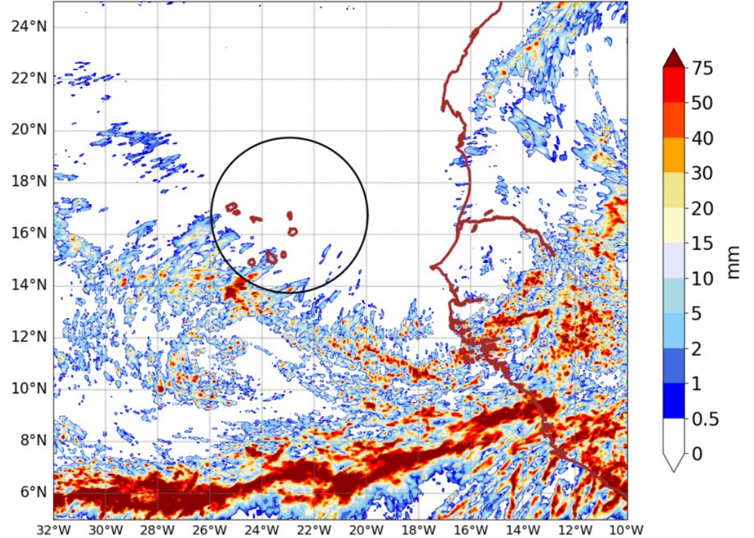
AROME25 20240921-00-UTC -ech(24h)
