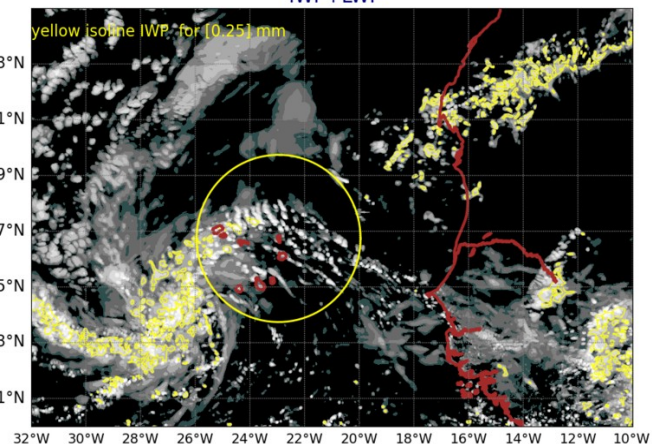
AROME25 20240924-12-UTC -ech(60h) IWP+LWP
