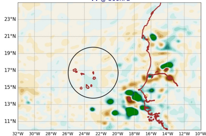
AROME25 20240922-12-UTC -ech(12h) VV @ 500hPa
