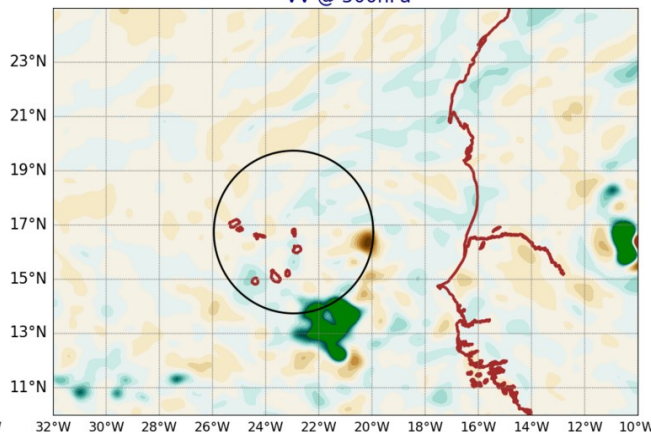
AROME25 20240923-12-UTC -ech(36h) VV @ 500hPa
