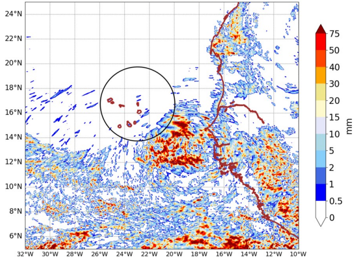
AROME25 20240924-12-UTC -ech(60h) RR cumulated over 24h
