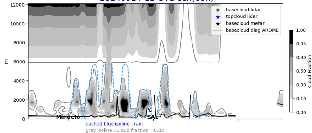
Cross section E/W @ 17.5N 20240924-12-UTC ech(60h)
