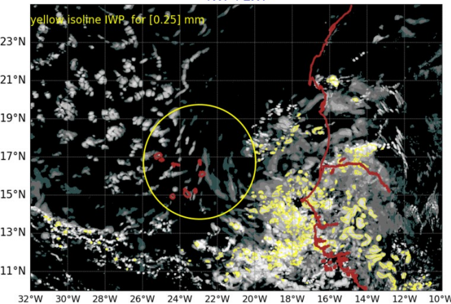
AROME25 20240922-12-UTC -ech(12h) IWP+LWP
