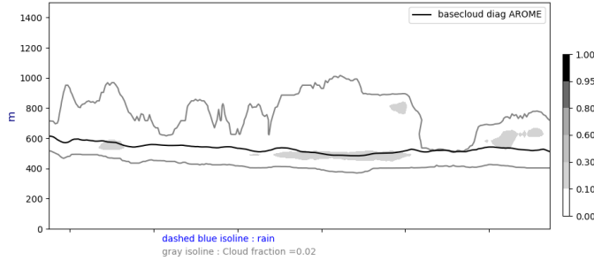
Cross section S/N @ -22W 20240922-12-UTC ech(12h)
