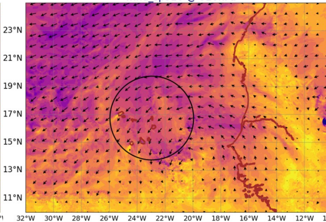
AROME25 20240923-12-UTC -ech(36h) wind_sp920 @ 920hPa
