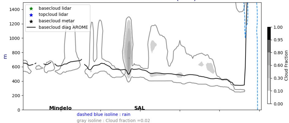
Cross section E/W @ 17.5N 20240922-12-UTC ech(12h)
