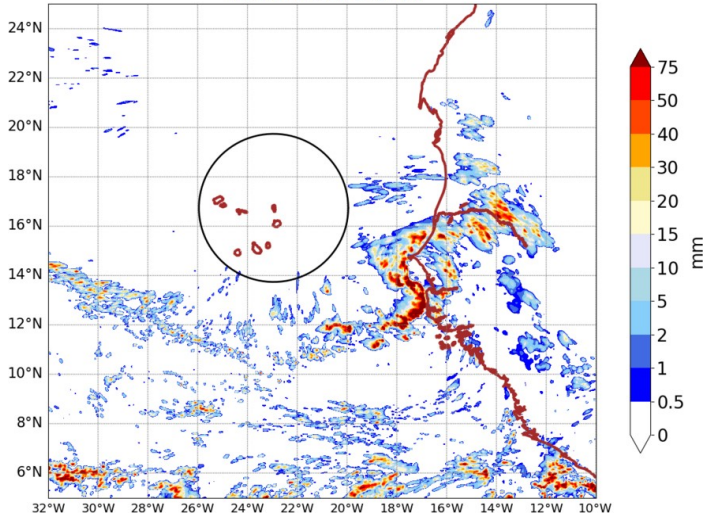
AROME25 20240922-15-UTC -ech(15h) RR cumulated over 6h
