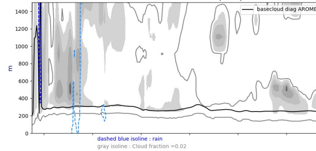
Cross section S/N @ -22W 20240923-12-UTC ech(36h)
