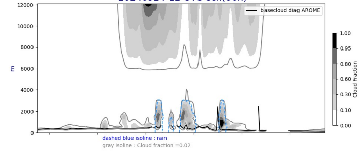
Cross section S/N @ -22W 20240924-12-UTC ech(60h)
