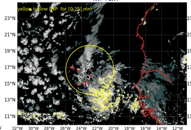
AROME25 20240923-12-UTC -ech(36h) IWP+LWP
