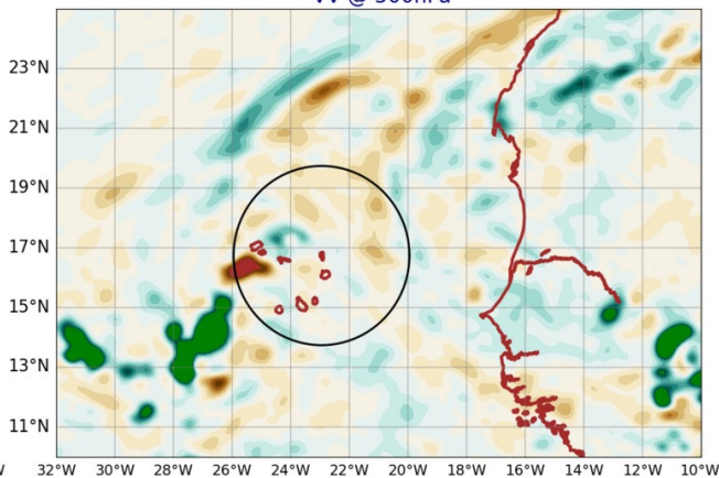
AROME25 20240924-12-UTC -ech(60h) VV @ 500hPa
