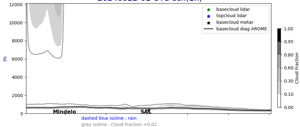
Cross section E/W @ 17.5N 20240922-01-UTC ech(1h)
