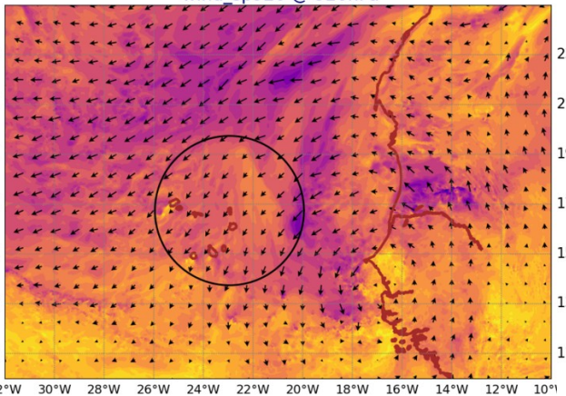
AROME25 20240922-12-UTC -ech(12h) wind_sp920 @ 920hPa
