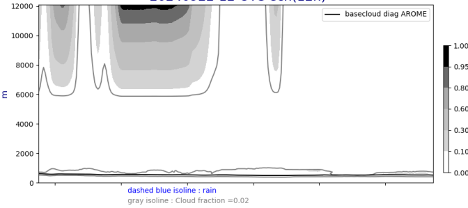
Cross section S/N @ -22W 20240922-12-UTC ech(12h)
