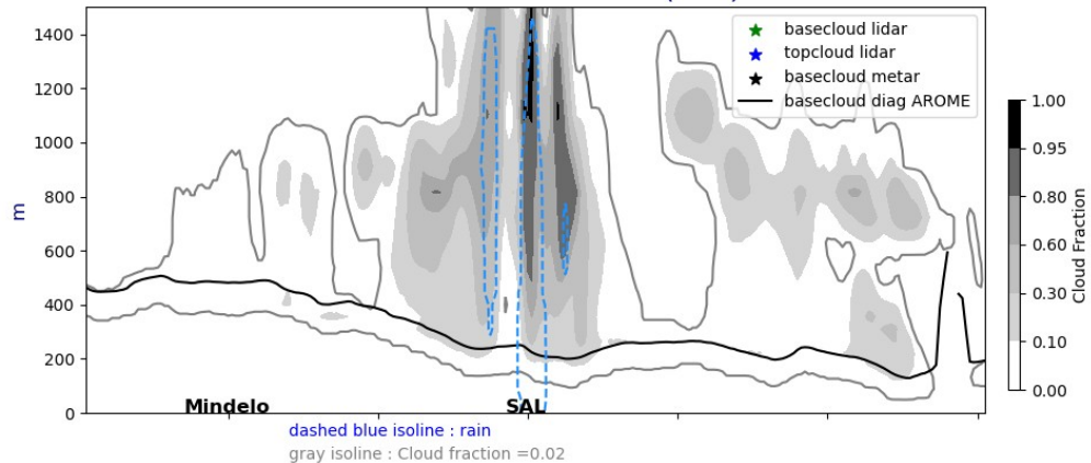
Cross section E/W @ 17.5N 20240923-12-UTC ech(36h)
