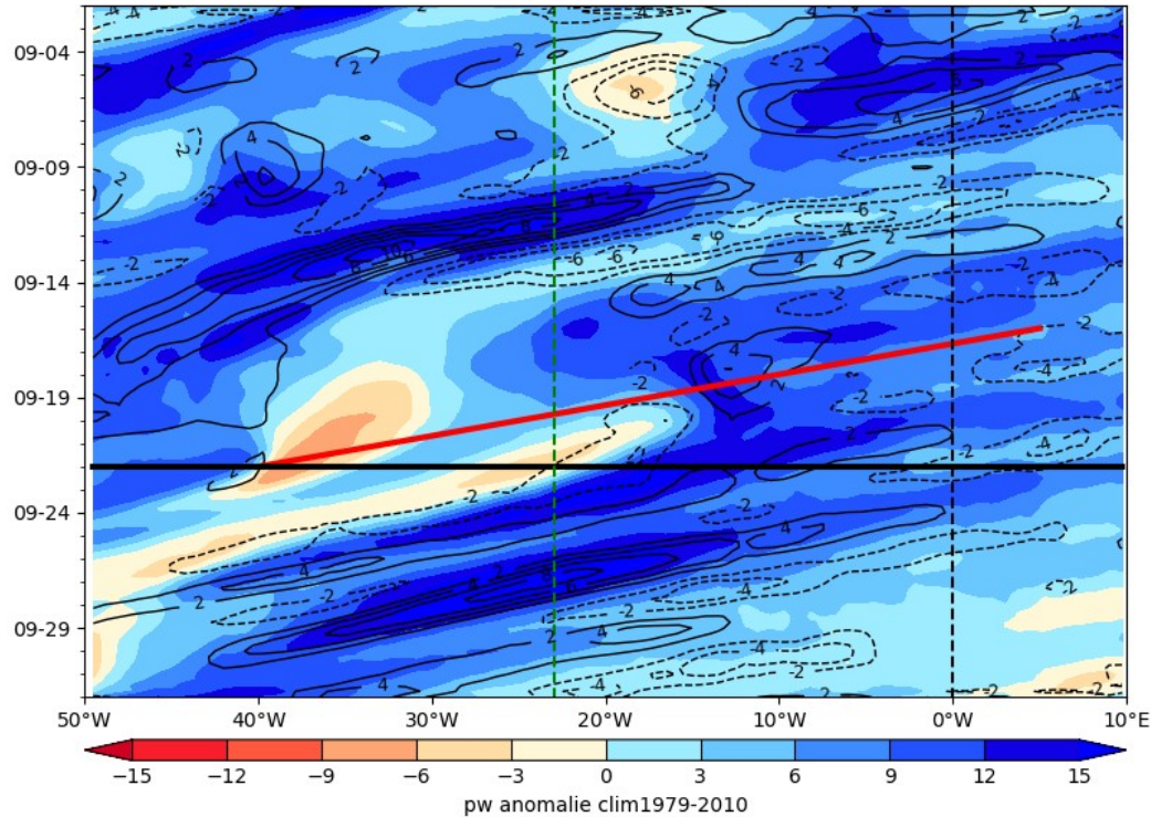
ECMWF PW (color) AND V at 925 hPa 2024-09-22
