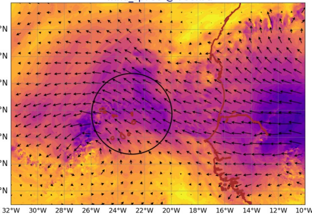
AROME25 20240924-12-UTC -ech(60h) wind_sp920 @ 920hPa
