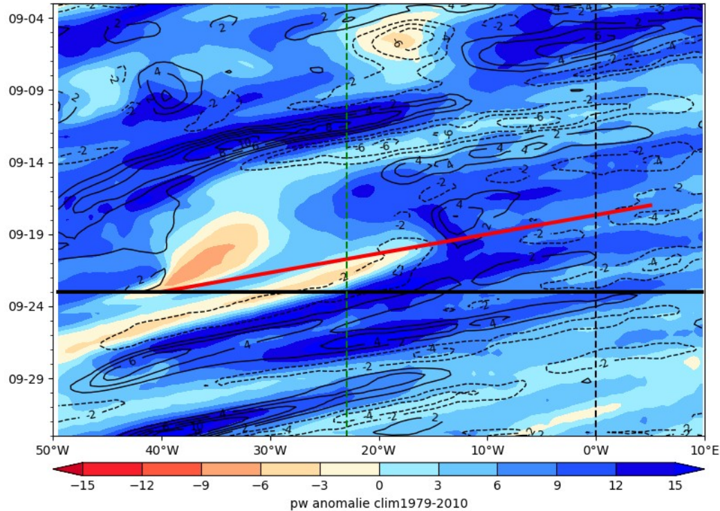
ECMWF PW (color) AND V at 925 hPa 2024-09-23
