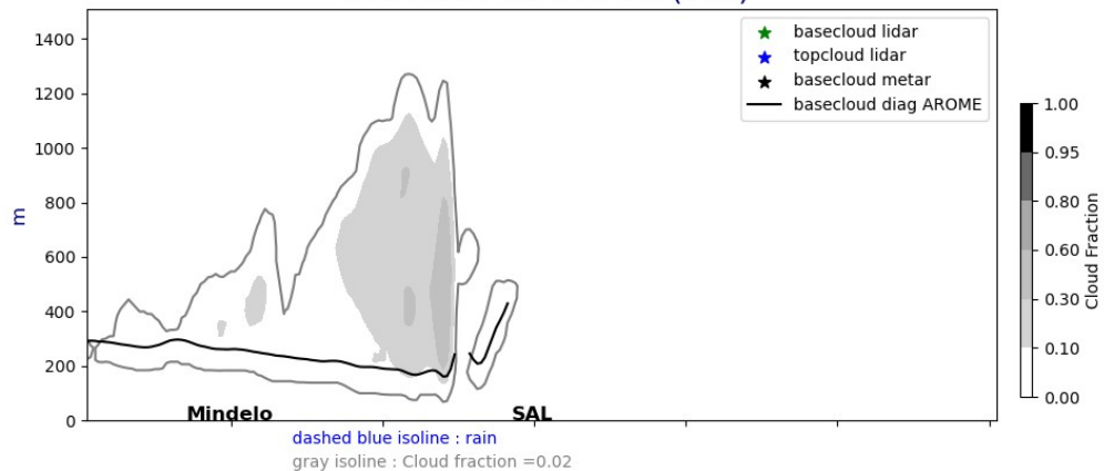
Cross section E/W @ 17.5N 20240924-12-UTC ech(36h)
