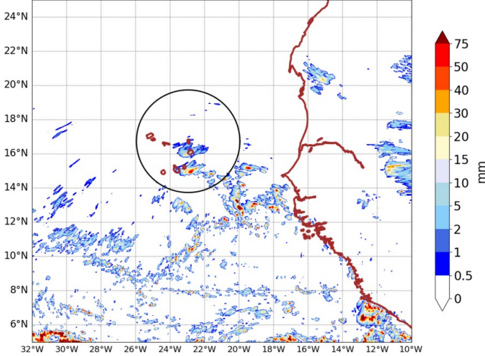
AROME25 20240923-15-UTC -ech(15h) RR cumulated over 6h
