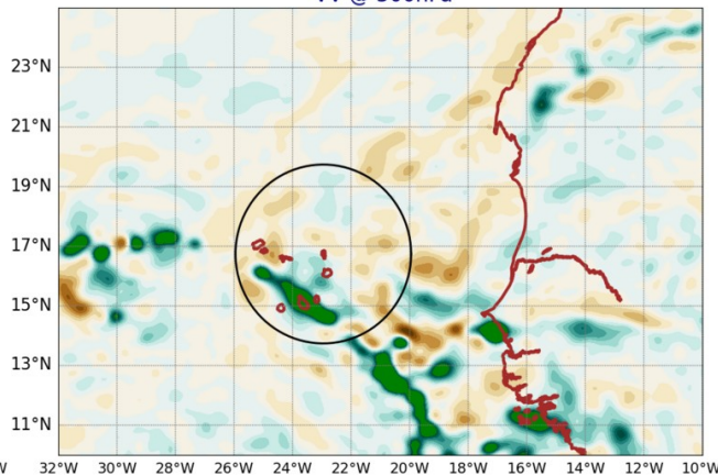
AROME25 20240925-12-UTC -ech(60h) VV @ 500hPa
