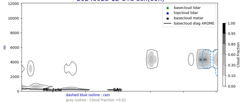
Cross section E/W @ 17.5N 20240925-12-UTC ech(60h)
