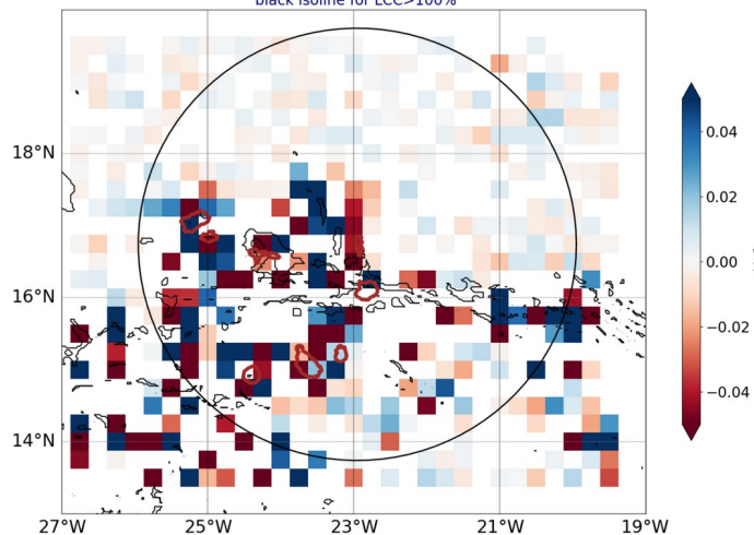
AROME25 regrid 0.25 20240924-12-UTC -ech(36h) blue for conv in subcloud layer black isoline for LCC>100%
