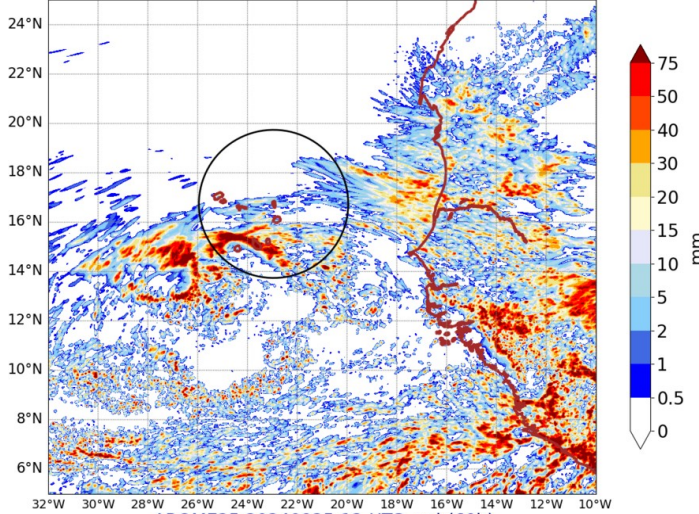
AROME25 20240925-12-UTC -ech(60h) RR cumulated over 24h
