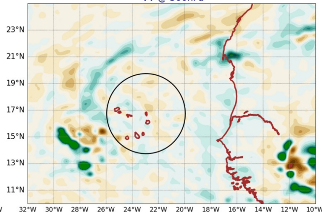
AROME25 20240924-12-UTC -ech(36h) VV @ 500hPa
