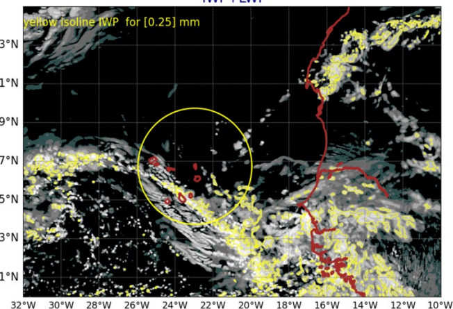
AROME25 20240925-12-UTC -ech(60h) IWP+LWP
