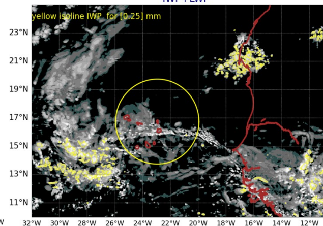
AROME25 20240924-12-UTC -ech(36h) IWP+LWP
