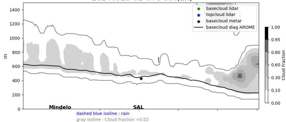
Cross section E/W @ 17.5N 20240923-01-UTC ech(1h)
