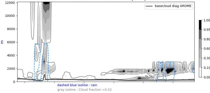
Cross section S/N @ -22W 20240923-12-UTC ech(12h)
