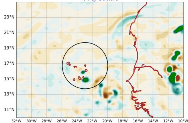
AROME25 20240923-12-UTC -ech(12h) VV @ 500hPa
