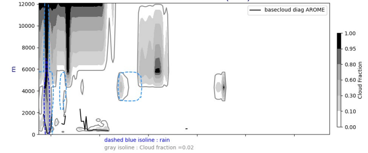
Cross section S/N @ -22W 20240925-12-UTC ech(60h)
