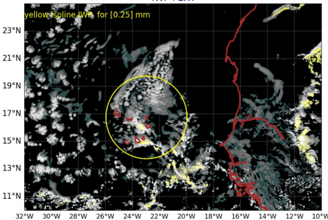
AROME25 20240923-12-UTC -ech(12h) IWP+LWP
