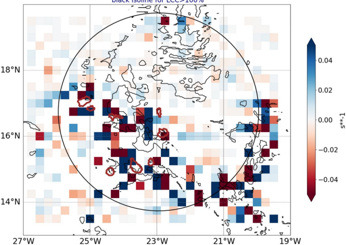
AROME25 regrid 0.25 20240923-12-UTC -ech(12h) blue for conv in subcloud layer black isoline for LCC>100%
