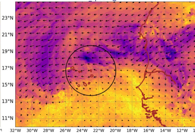
AROME25 20240924-12-UTC -ech(36h) wind_sp920 @ 920hPa
