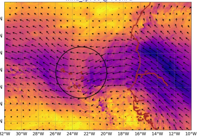
AROME25 20240925-12-UTC -ech(60h) wind_sp920 @ 920hPa
