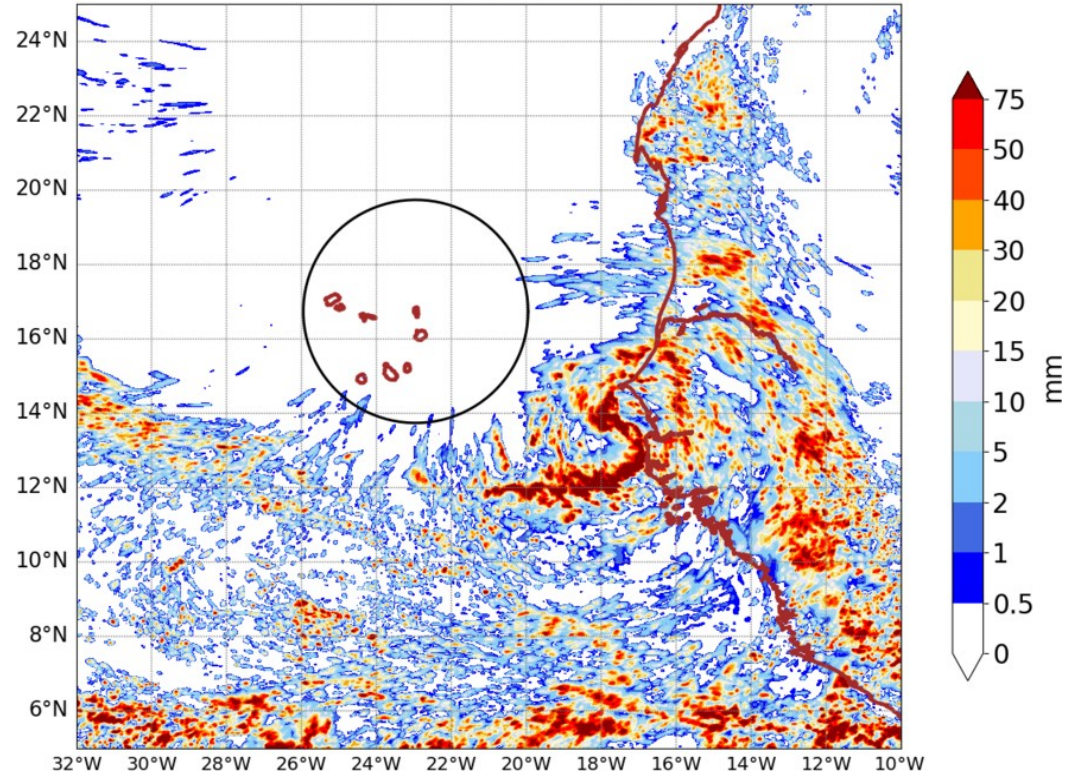
AROME25 20240923-00-UTC -ech(24h)
