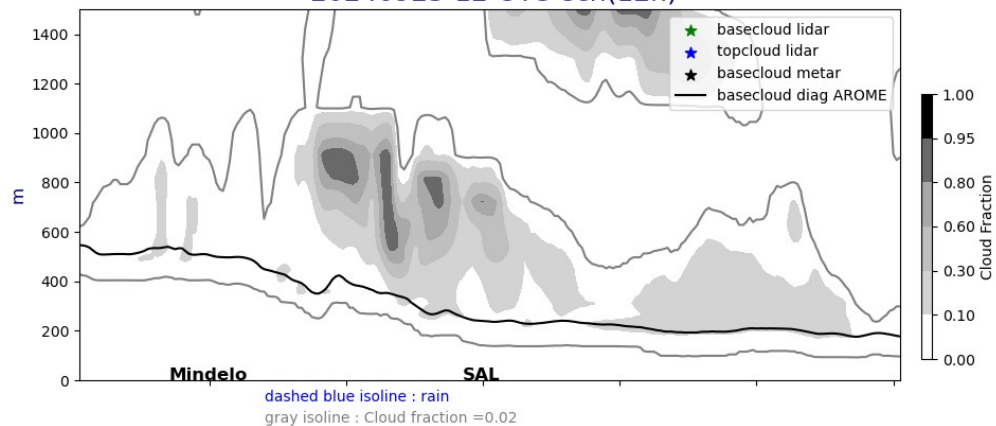
Cross section E/W @ 17.5N 20240923-12-UTC ech(12h)
