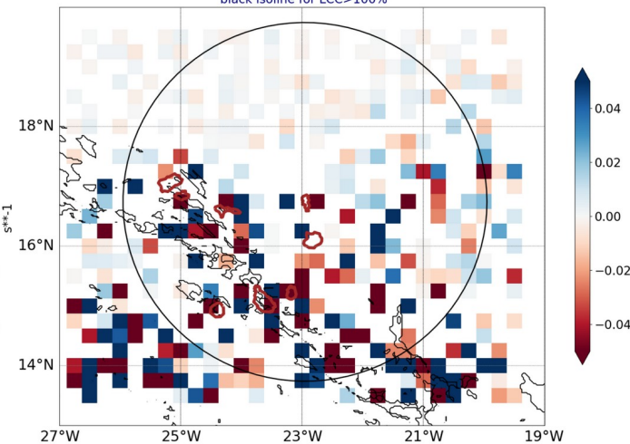
AROME25 regrid 0.25 20240925-12-UTC -ech(60h) blue for conv in subcloud layer black isoline for LCC>100%
