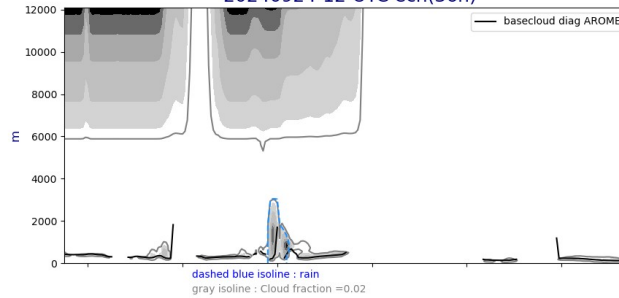
Cross section S/N @ -22W 20240924-12-UTC ech(36h)
