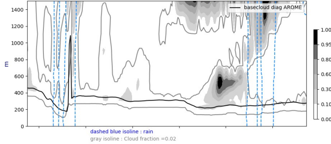
Cross section S/N @ -22W 20240923-12-UTC ech(12h)
