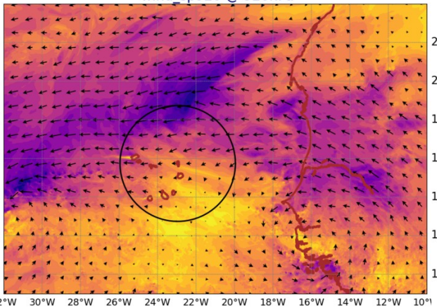
AROME25 20240925-12-UTC -ech(12h) wind_sp920 @ 920hPa
