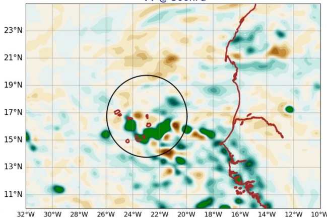
AROME25 20240926-12-UTC -ech(36h) VV @ 500hPa
