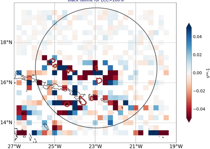
AROME25 regrid 0.25 20240925-12-UTC -ech(12h) blue for conv in subcloud layer black isoline for LCC>100%
