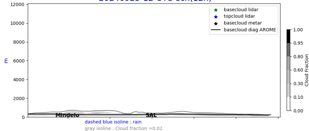
Cross section E/W @ 17.5N 20240925-12-UTC ech(12h)
