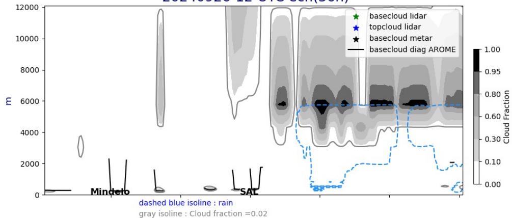
Cross section E/W @ 17.5N 20240926-12-UTC ech(36h)
