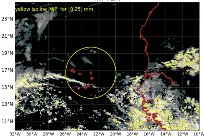
AROME25 20240925-12-UTC -ech(12h) IWP+LWP
