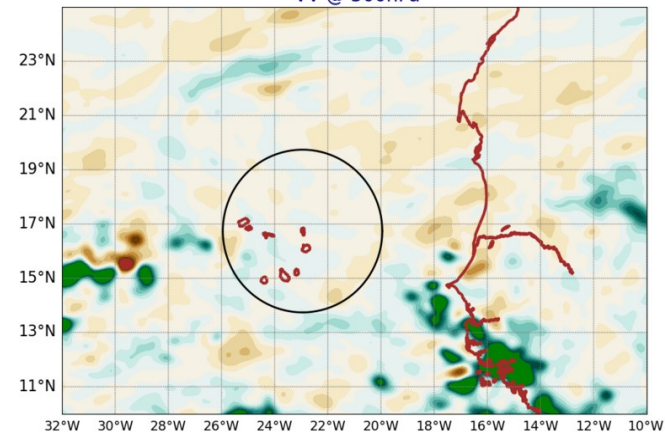
AROME25 20240925-12-UTC -ech(12h) VV @ 500hPa
