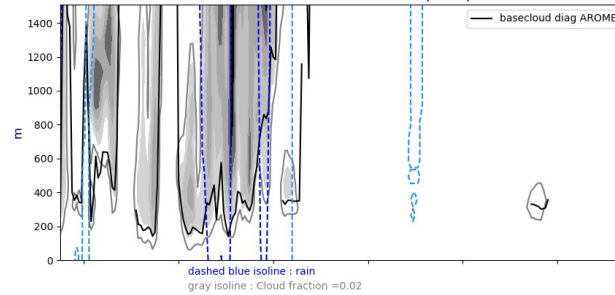
Cross section S/N @ -22W 20240926-12-UTC ech(36h)
