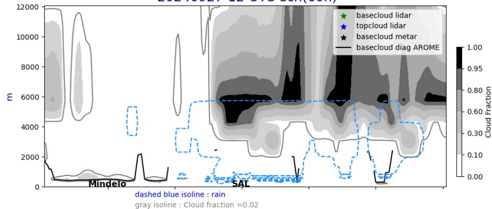
Cross section E/W @ 17.5N 20240927-12-UTC ech(60h)
