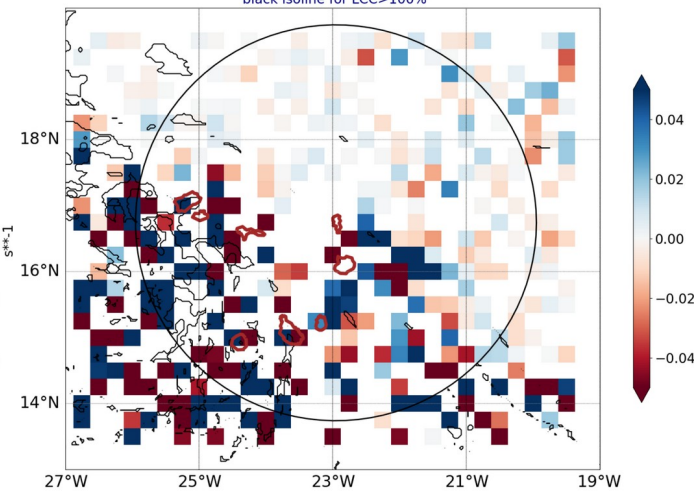
AROME25 regrid 0.25 20240927-12-UTC -ech(60h) blue for conv in subcloud layer black isoline for LCC>100%
