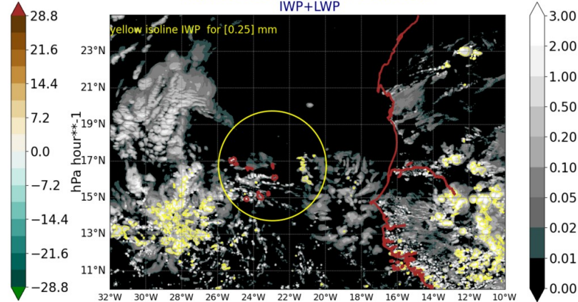
AROME25 20240924-15-UTC -ech(15h) IWP+LWP
