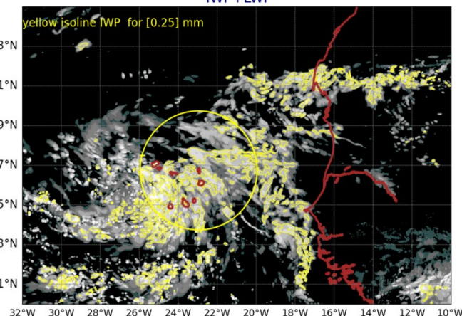
AROME25 20240927-12-UTC -ech(60h) IWP+LWP
