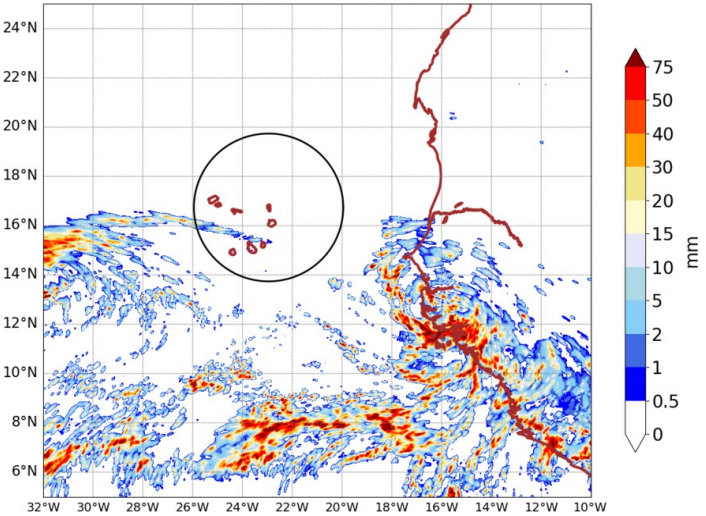
AROME25 20240925-15-UTC -ech(15h) RR cumulated over 6h
