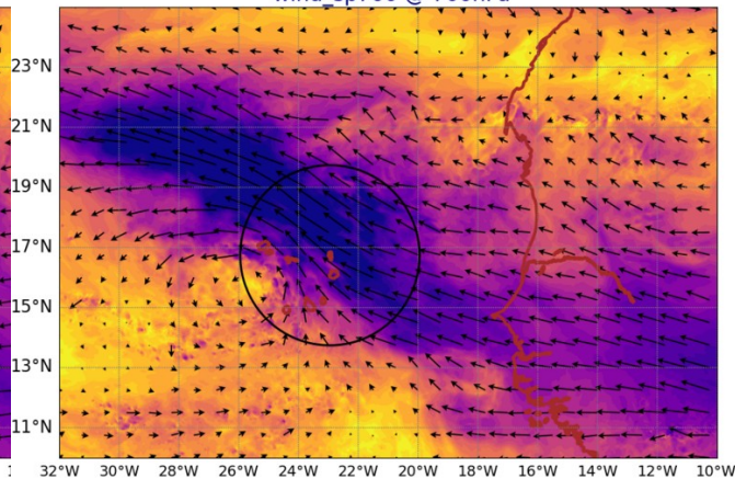
AROME25 20240927-12-UTC -ech(60h) wind_sp920 @ 920hPa
