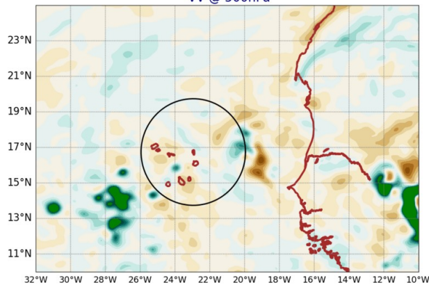
AROME25 20240924-12-UTC -ech(12h) VV @ 500hPa
