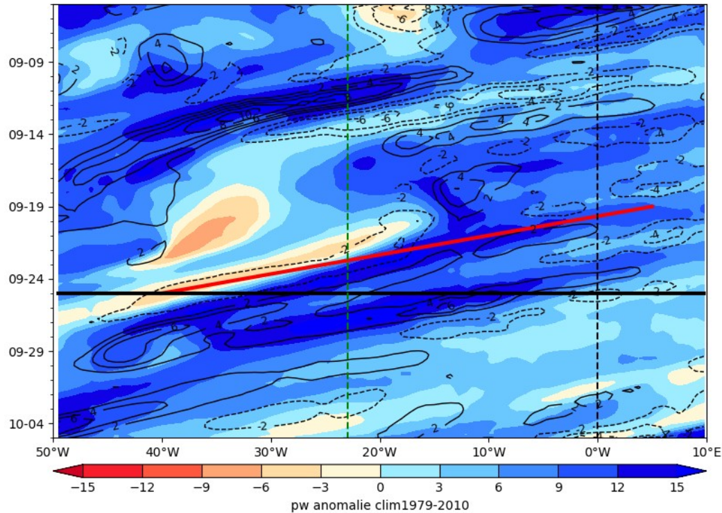
ECMWF PW (color) AND V at 925 hPa 2024-09-25
