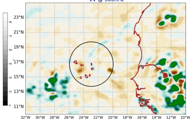
AROME25 20240924-15-UTC -ech(15h) VV @ 500hPa
