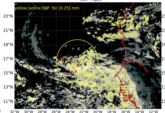
AROME25 20240926-12-UTC -ech(36h) IWP+LWP
