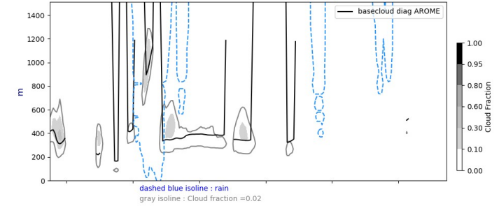
Cross section S/N @ -22W 20240927-12-UTC ech(60h)
