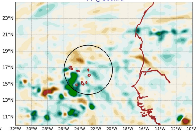
AROME25 20240927-12-UTC -ech(60h) VV @ 500hPa
