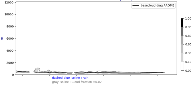
Cross section S/N @ -22W 20240925-12-UTC ech(12h)
