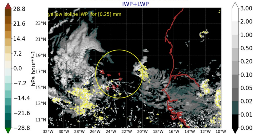
AROME25 20240924-12-UTC -ech(12h) IWP+LWP
