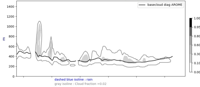
Cross section S/N @ -22W 20240925-12-UTC ech(12h)
