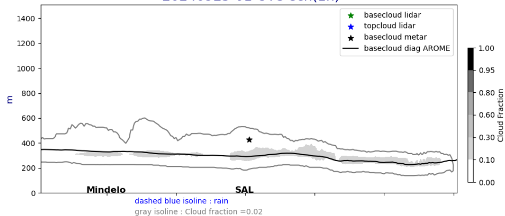
Cross section E/W @ 17.5N 20240925-01-UTC ech(1h)
