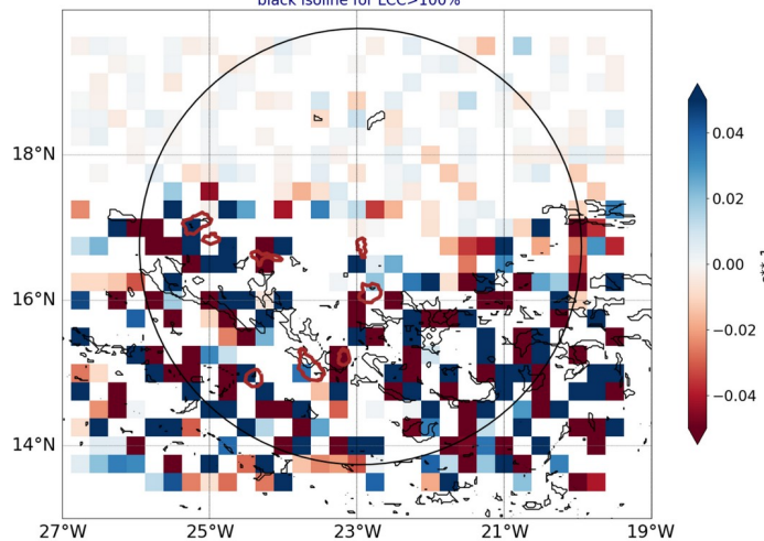
AROME25 regrid 0.25 20240926-12-UTC -ech(36h) blue for conv in subcloud layer black isoline for LCC>100%
