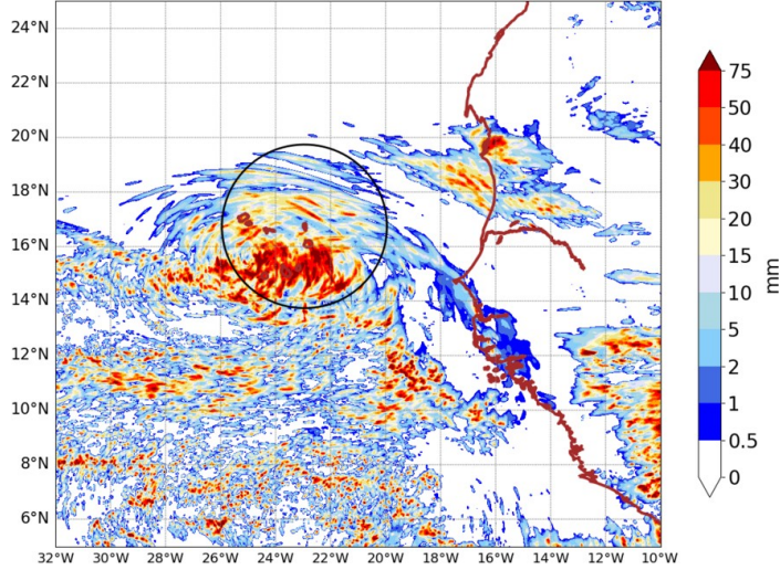
AROME25 20240927-12-UTC -ech(60h) RR cumulated over 24h
