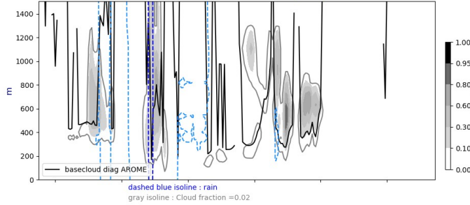
Cross section S/N @ -22W 20240927-12-UTC ech(12h)
