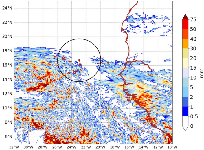
AROME25 20240929-12-UTC -ech(60h) RR cumulated over 24h
