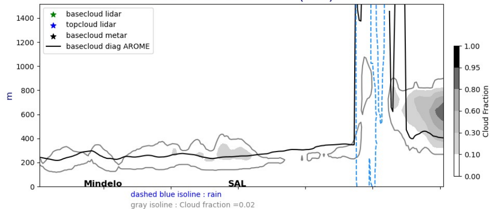
Cross section E/W @ 17.5N 20240928-12-UTC ech(36h)
