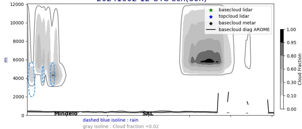
Cross section E/W @ 17.5N 20241002-12-UTC ech(60h)
