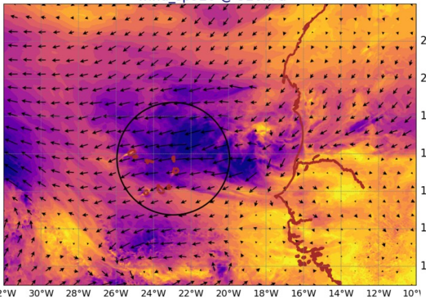
AROME25 20240930-12-UTC -ech(12h) wind_sp920 @ 920hPa
