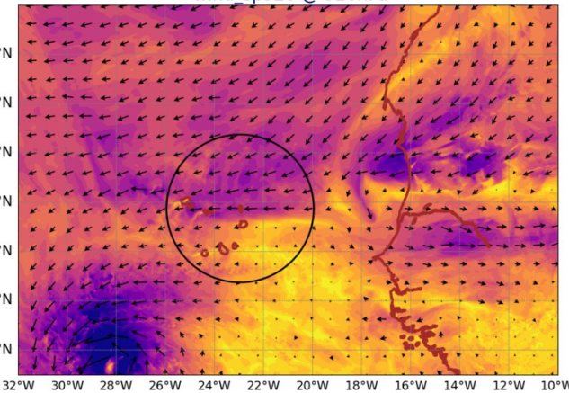
AROME25 20241002-12-UTC -ech(60h) wind_sp920 @ 920hPa
