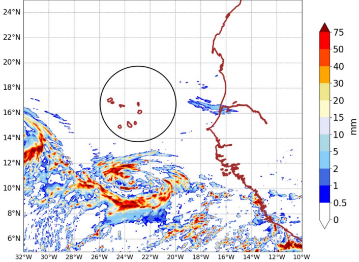
AROME25 20240930-15-UTC -ech(15h) RR cumulated over 6h
