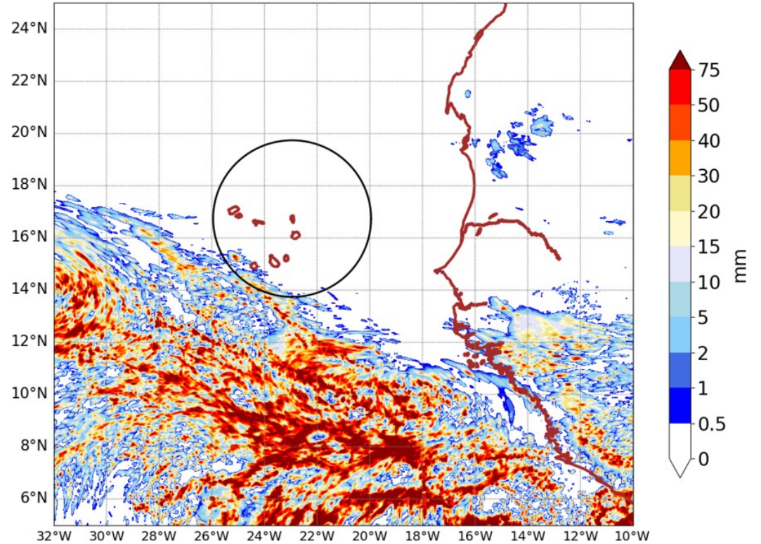
AROME25 20240930-00-UTC -ech(24h)
