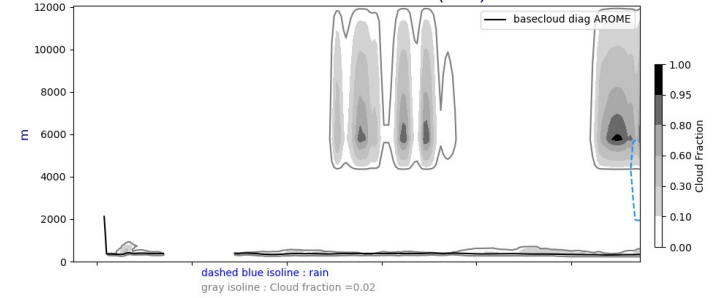
Cross section S/N @ -22W 20241002-12-UTC ech(60h)
