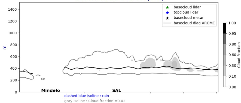
Cross section E/W @ 17.5N 20241001-12-UTC ech(36h)
