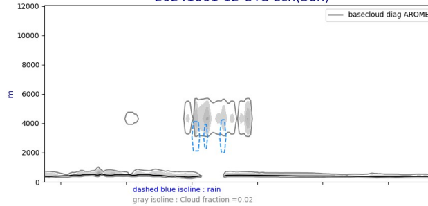
Cross section S/N @ -22W 20241001-12-UTC ech(36h)
