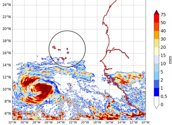
AROME25 20241002-12-UTC -ech(60h) RR cumulated over 24h
