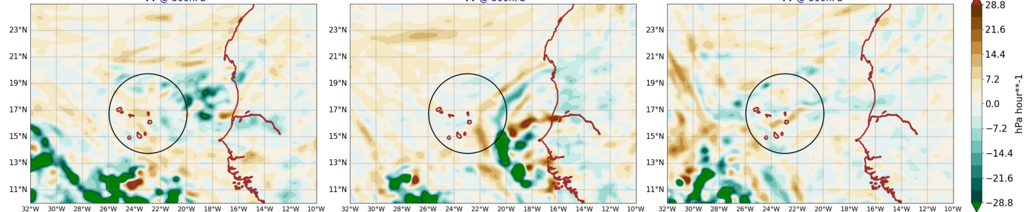
AROME25 20240930-12-UTC -ech(12h) VV @ 500hPa
