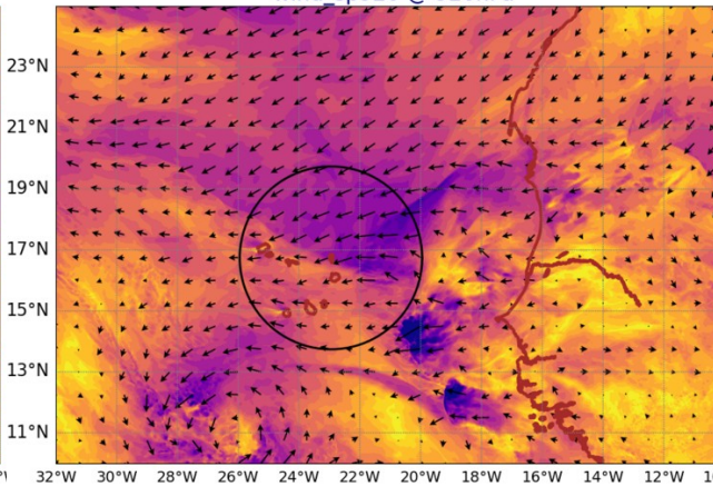
AROME25 20241001-12-UTC -ech(36h) wind_sp920 @ 920hPa
