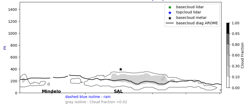
Cross section E/W @ 17.5N 20240930-01-UTC ech(1h)
