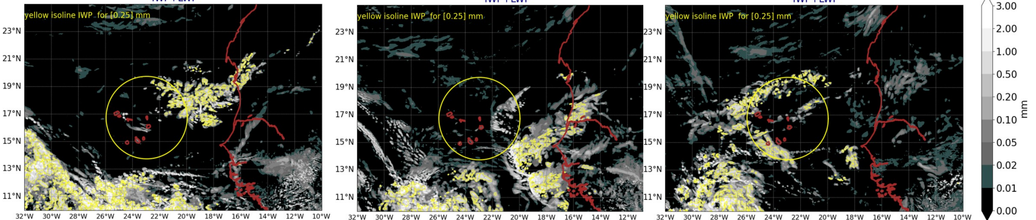
AROME25 20240930-12-UTC -ech(12h) IWP+LWP
