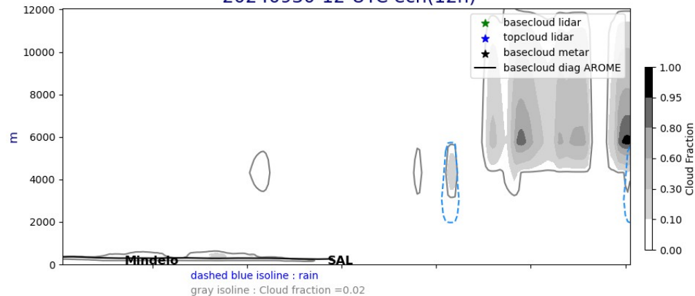
Cross section E/W @ 17.5N 20240930-12-UTC ech(12h)
