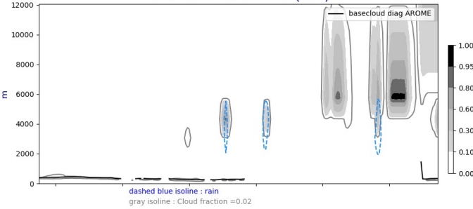
Cross section S/N @ -22W 20240930-12-UTC ech(12h)
