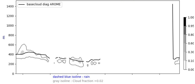
Cross section S/N @ -22W 20240930-12-UTC ech(12h)
