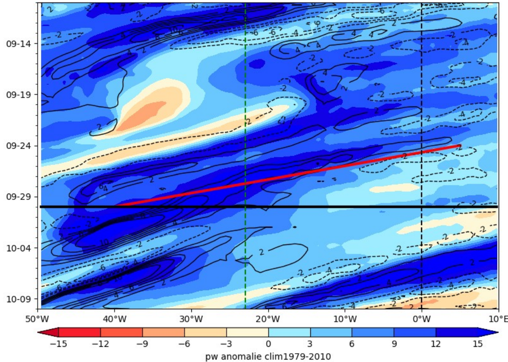
ECMWF PW (color) AND V at 925 hPa 2024-09-30
